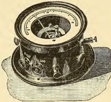
FIG. 103.—Edelmann galvanometer.
